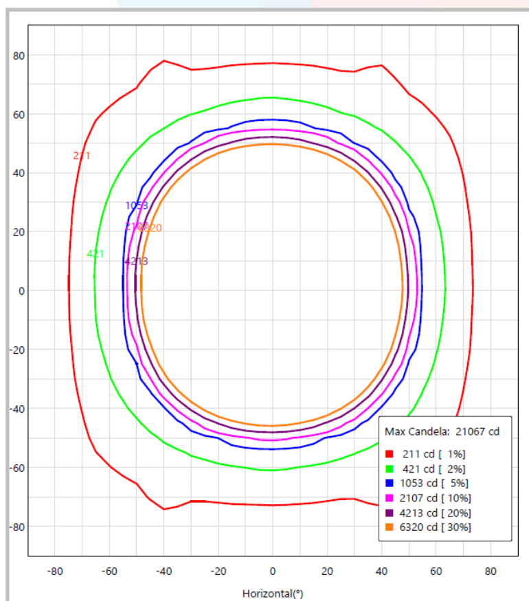
ISOCANDELA
